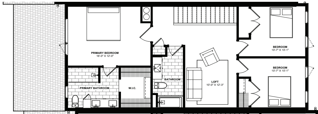
MAIN FLOOR
