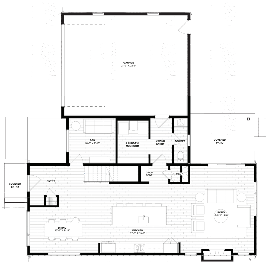
MAIN FLOOR
