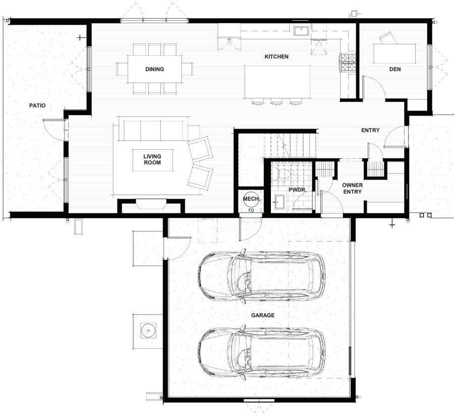
MAIN FLOOR
