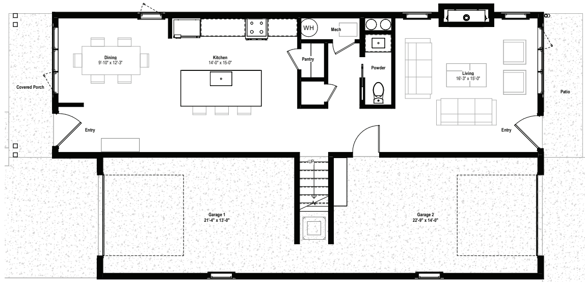
MAIN FLOOR
